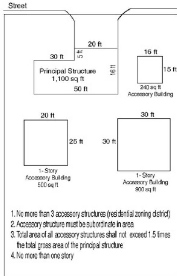
Figure 151.113: Accessory Structures
