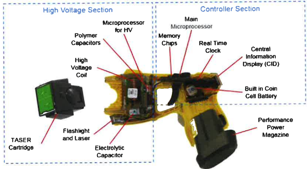
Figure 3: Cutaway View of TASER X26P with Labeled Internal Components
