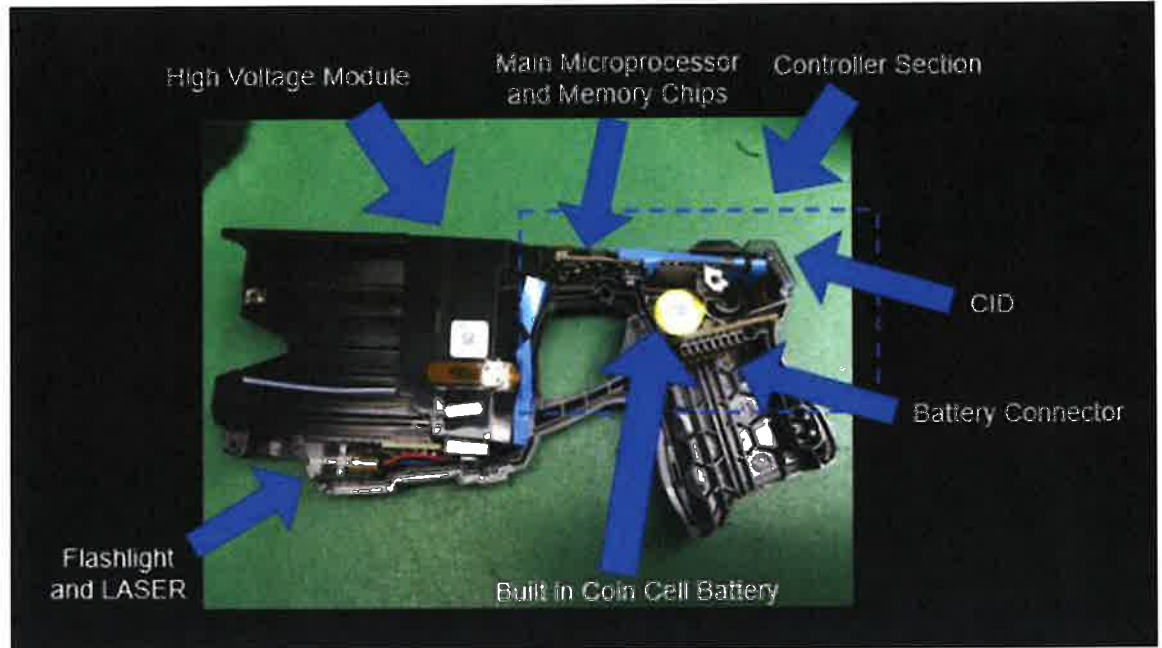
Figure 2: Cutaway View of TASER X2 with Labeled Internal Components
